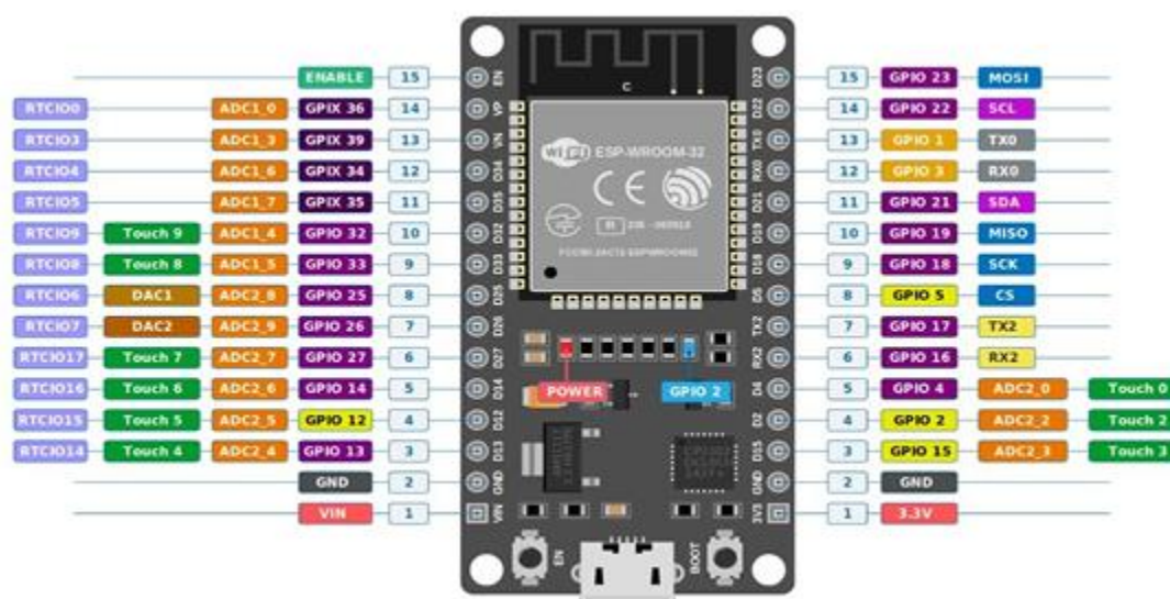
Fig. 4.2 ESP32 MICROCONTROLLER
