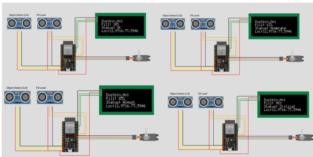
Fig. 5.2 Wokwi simulation prototype of smart waste bin at different fill levels.
