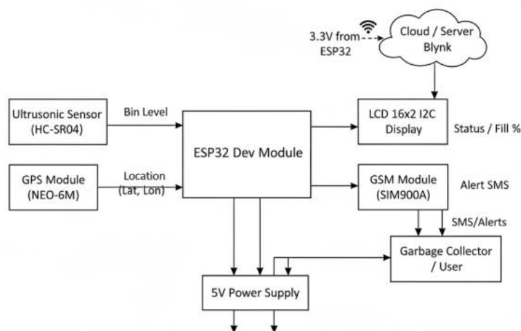
Fig. 4.8 Schematic representation of hardware implementation of the system.
