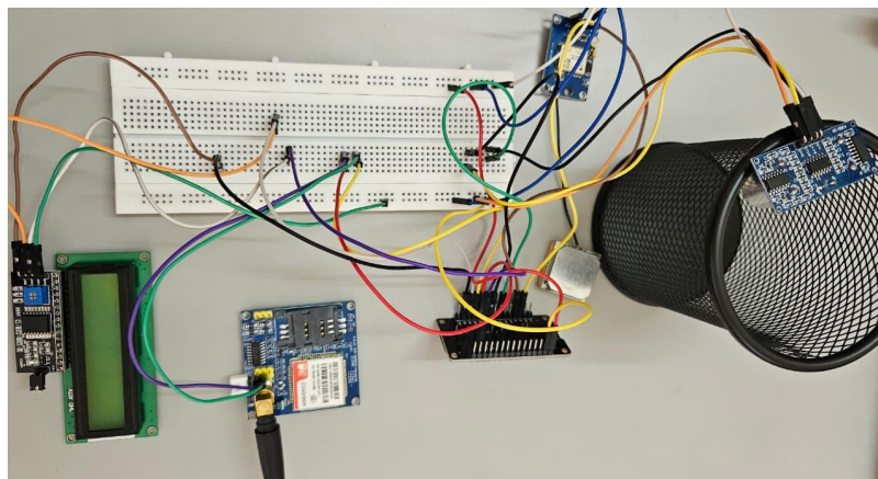
Fig. 5.1 Experimental Setup of ESP32 Smart Waste Bin Node.
