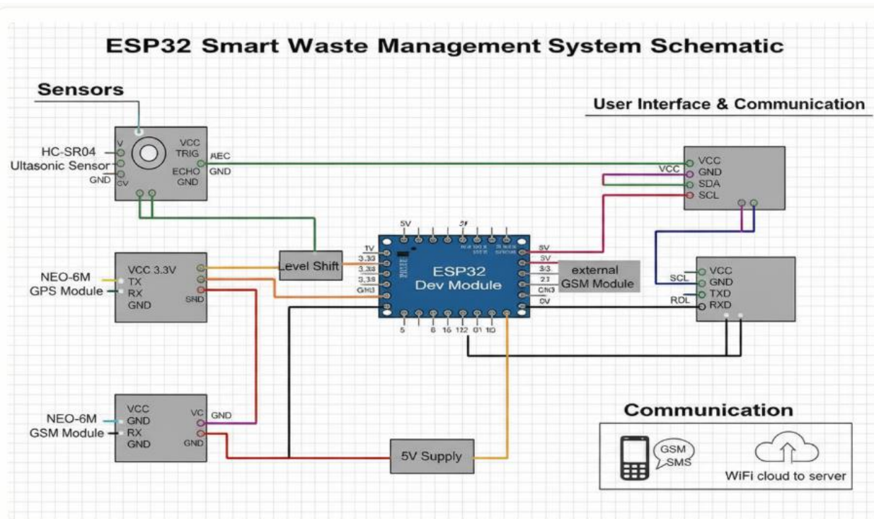
Fig. 4.8 Schematic representation of ESP32-based smart waste bin node.
