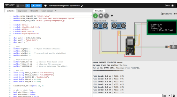
Fig. 4.9 Wokwi simulation of the ESP32-based smart waste bin node.
